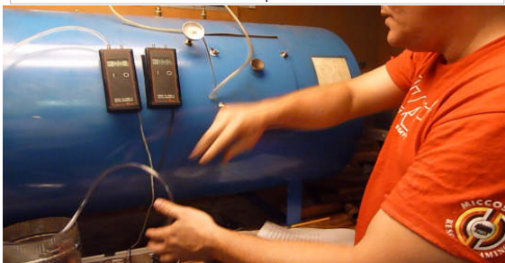
Digital Manometers
